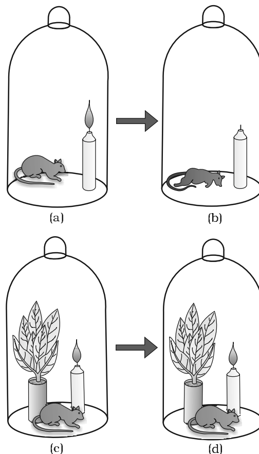
Figure 13.1 Priestley's experiment
