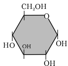
C_6H_{12}O_6 (Glucose)
